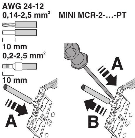
Figure 7 Push-in connection
