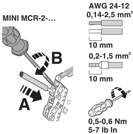
Figure 6 Screw connection
